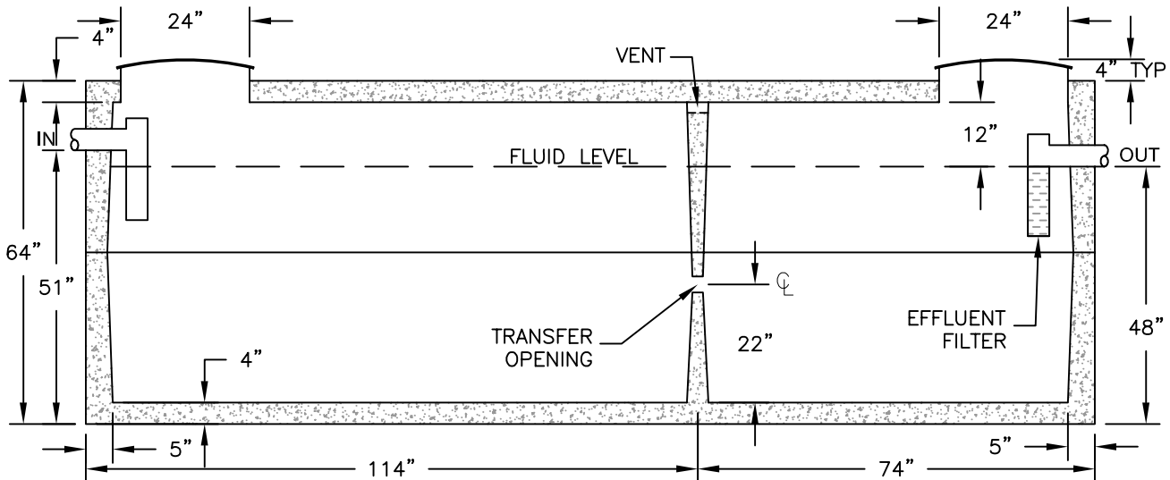
Section A - A' SIDE VIEW
